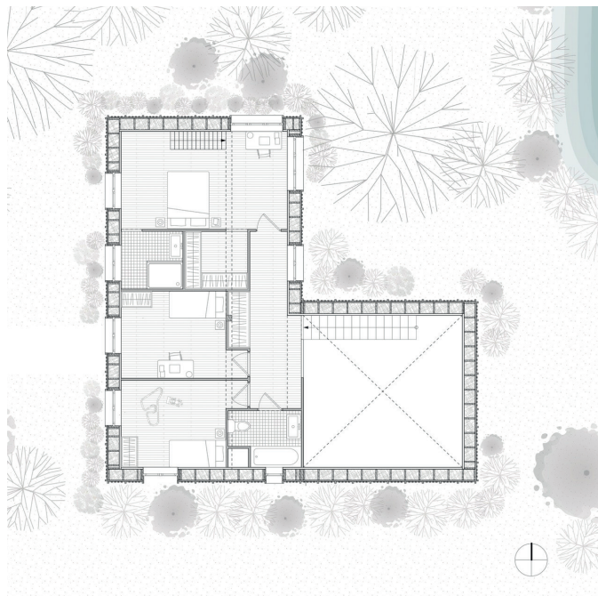
Plan R+1
