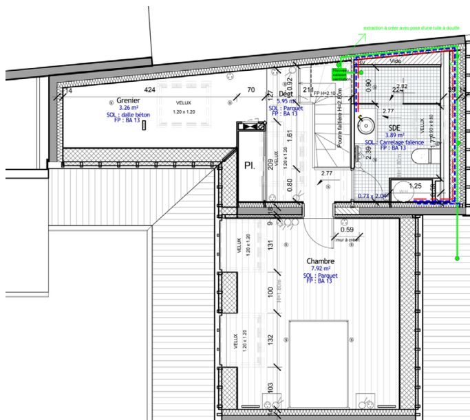
Plan R+comble - 1.50
