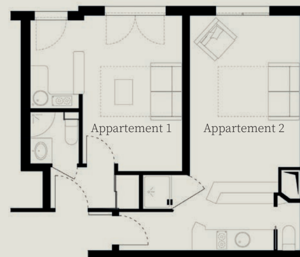
Plan existant
