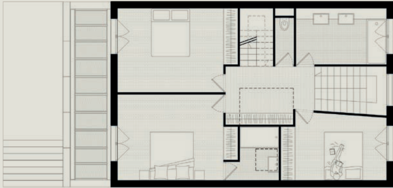
Plan R+1
