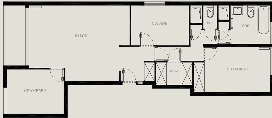
Plan existant
